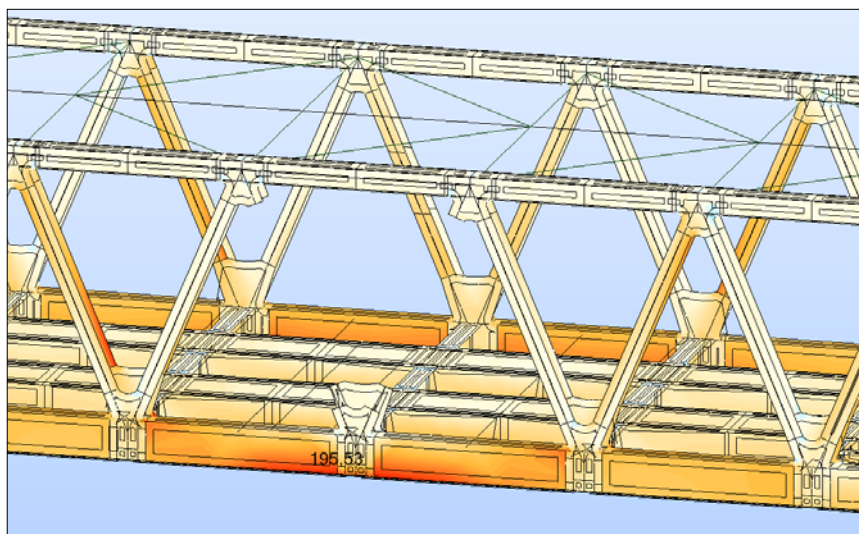
Figure 11: One of the accidental load cases that has been studied.
